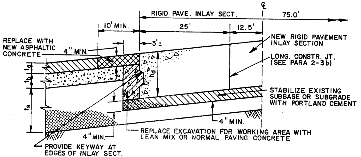
TRANSVERSE SECTION SHOWING CONSTRUCTION OF RIGID PAVEMENT INLAY SECTION IN RUNWAYS
