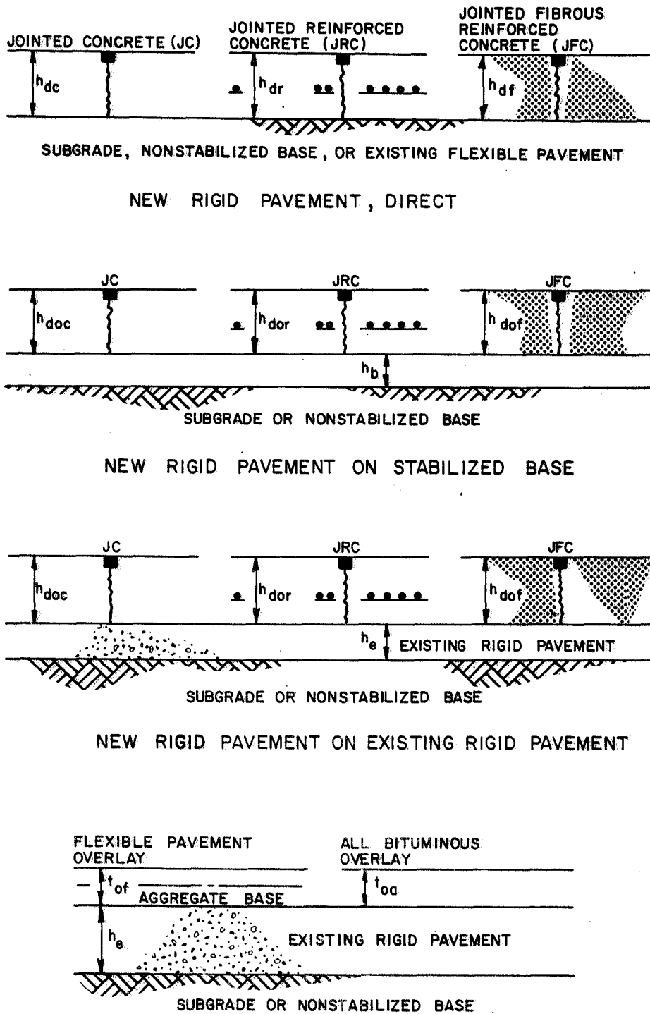
ASPHALTIC OVERLAY ON EXISTING RIGID PAVEMENT
